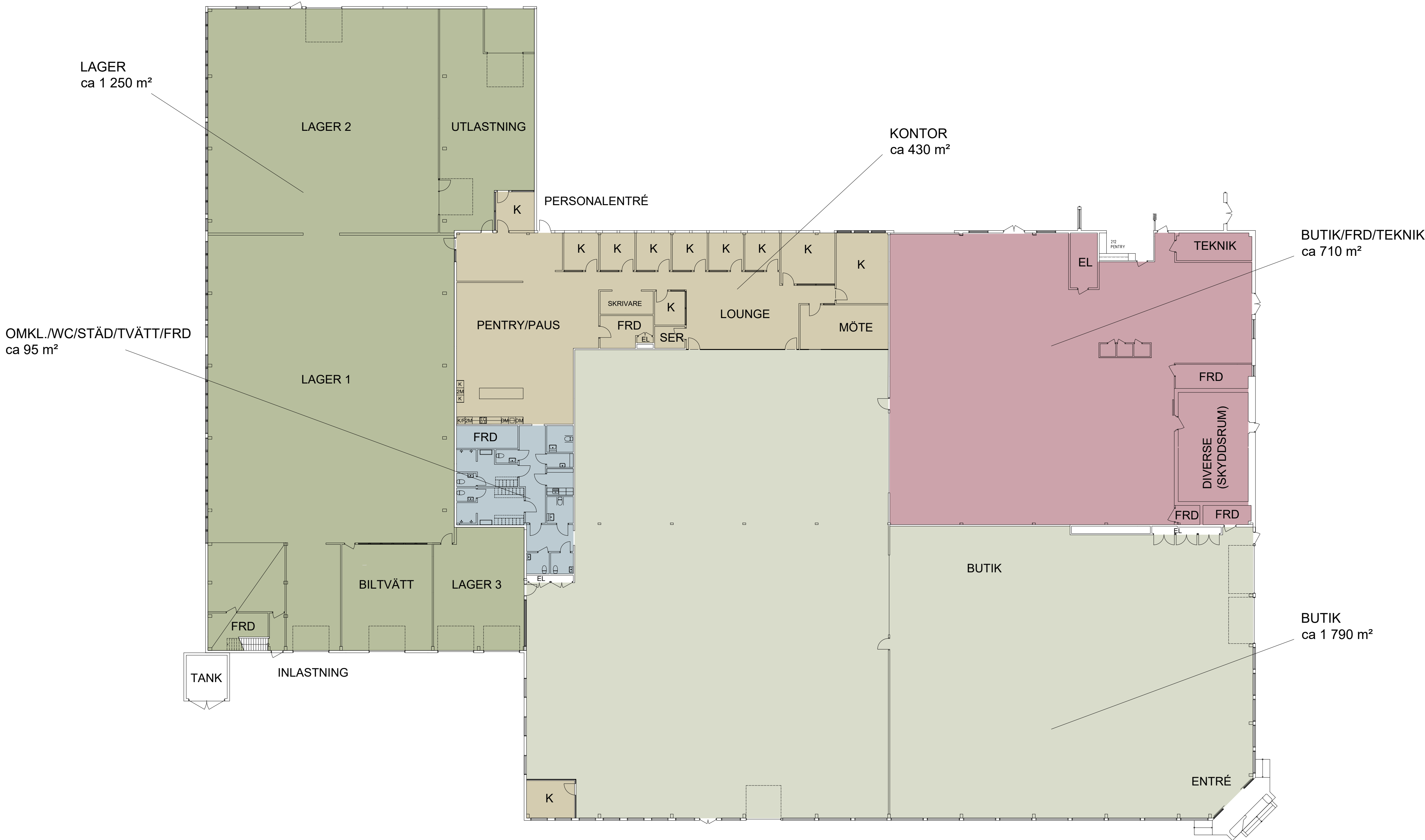
PLAN 1 skala 1:200
