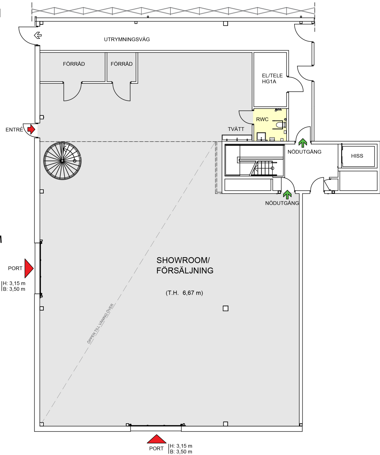
Markplan SHOWROOM
